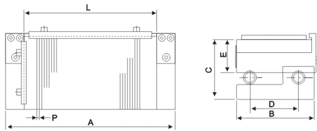
Structural Dimension of Lockable & Single Tiltable Type Chuck
